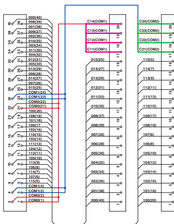
VSF-FLK40/SPT1,5/OM3-J (1270518)
