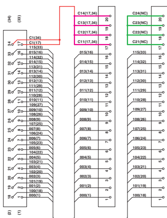
VSF-FLK34/SPT1,5/KV-J (1253685)
